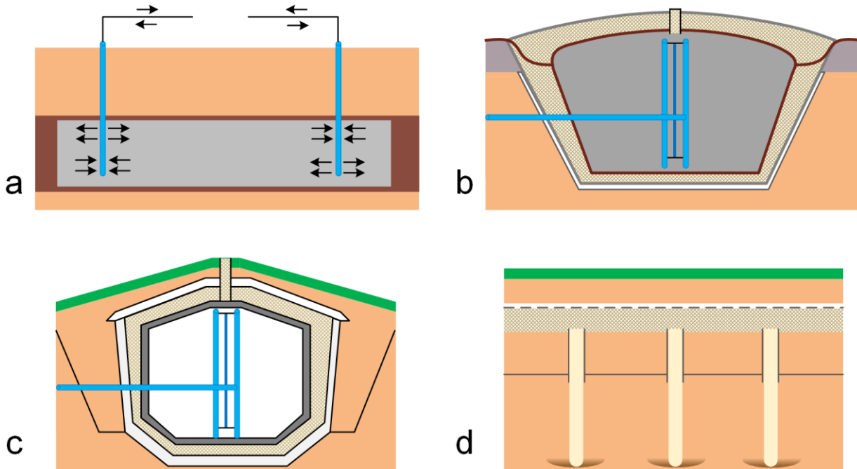
Seasonal storage methods of solar heat: A and D – underground reservoirs; B and C – up-underground storages
